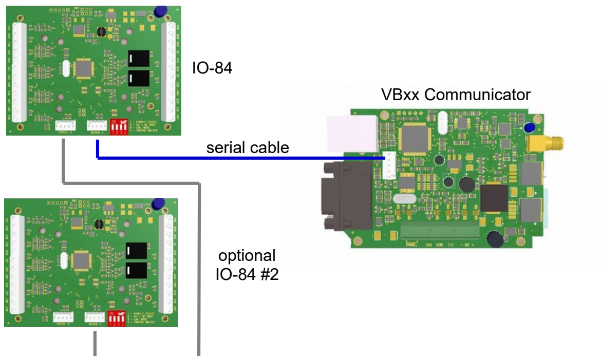
Figure 1.: Normal operation, one communicator with 1 or 2 IO-84 modules
